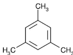
1,3,5-Trimethylbenzol
