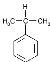
iso-Propylbenzol
